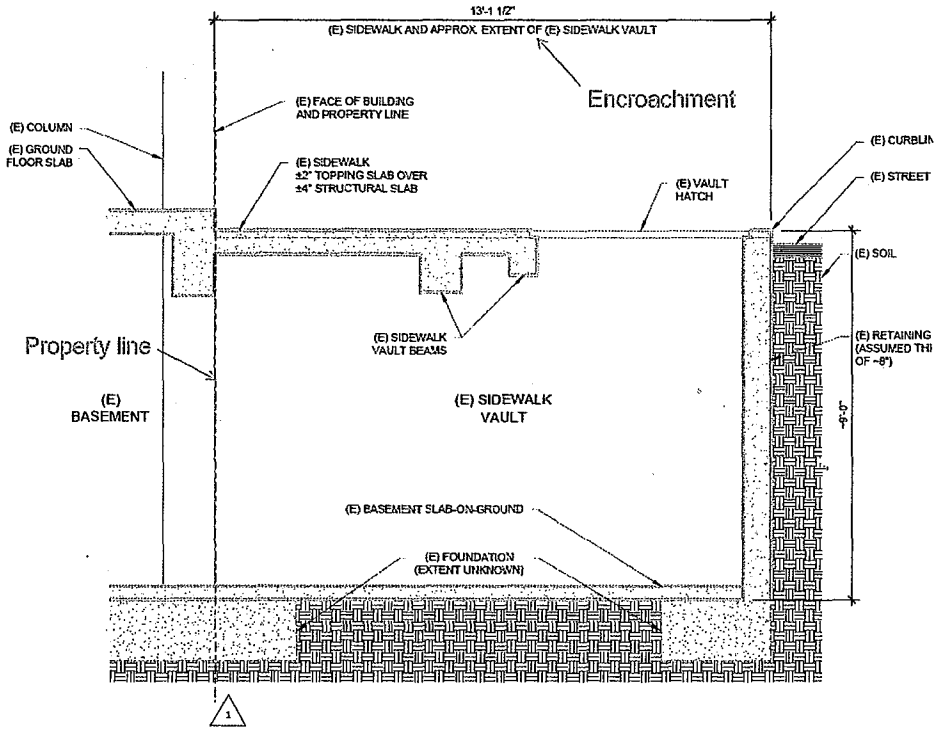
3 VAULT AT HATCH SCALE: 1/2" = 1'-0"
