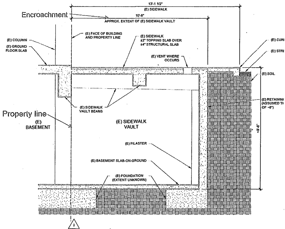
2 TYP. VAULT ON FRANKLIN STREET SCALE: 1/2" = 1'-0"
