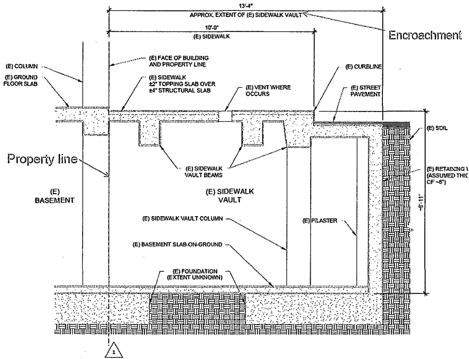
1 TYP. VAULT ON 19th STREET SCALE: 1/2" = 1'-0"
