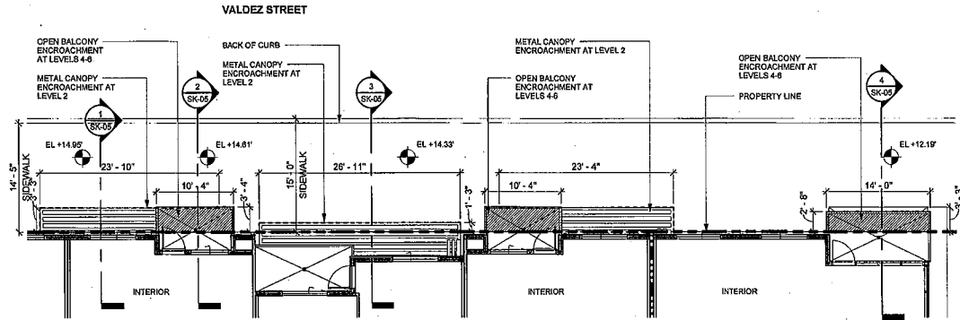
1 VALDEZ STREET PARTIAL PLAN 1/8" = 1'-0"
