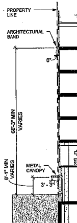
2 SECTION 2 1/16" = 1'-0"
