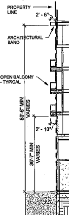
4 SECTION 4 1/16" = 1'-0"
