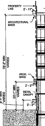
3 SECTION 3 1/16" = 1'-0"
