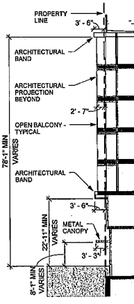
1 SECTION 1 1/16" = 1'-0"
