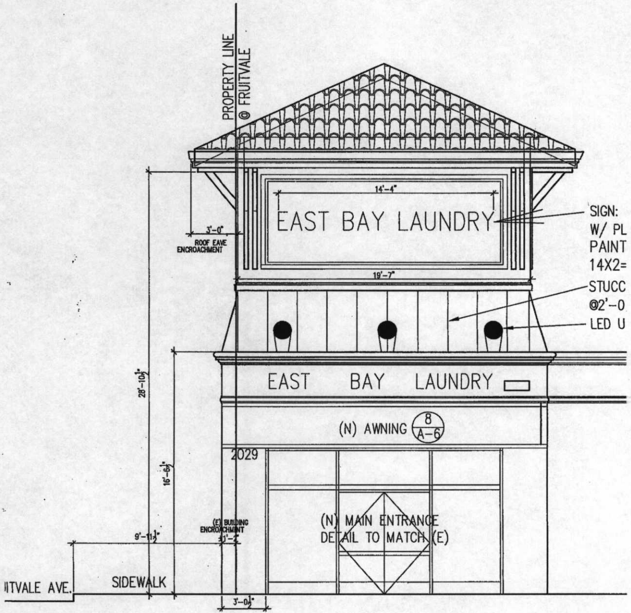
ENCROACHMENT SECTION
