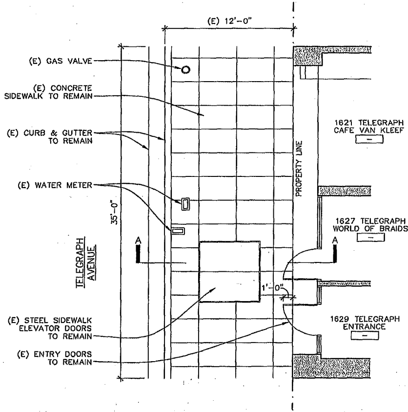
SIDEWALK PLAN
