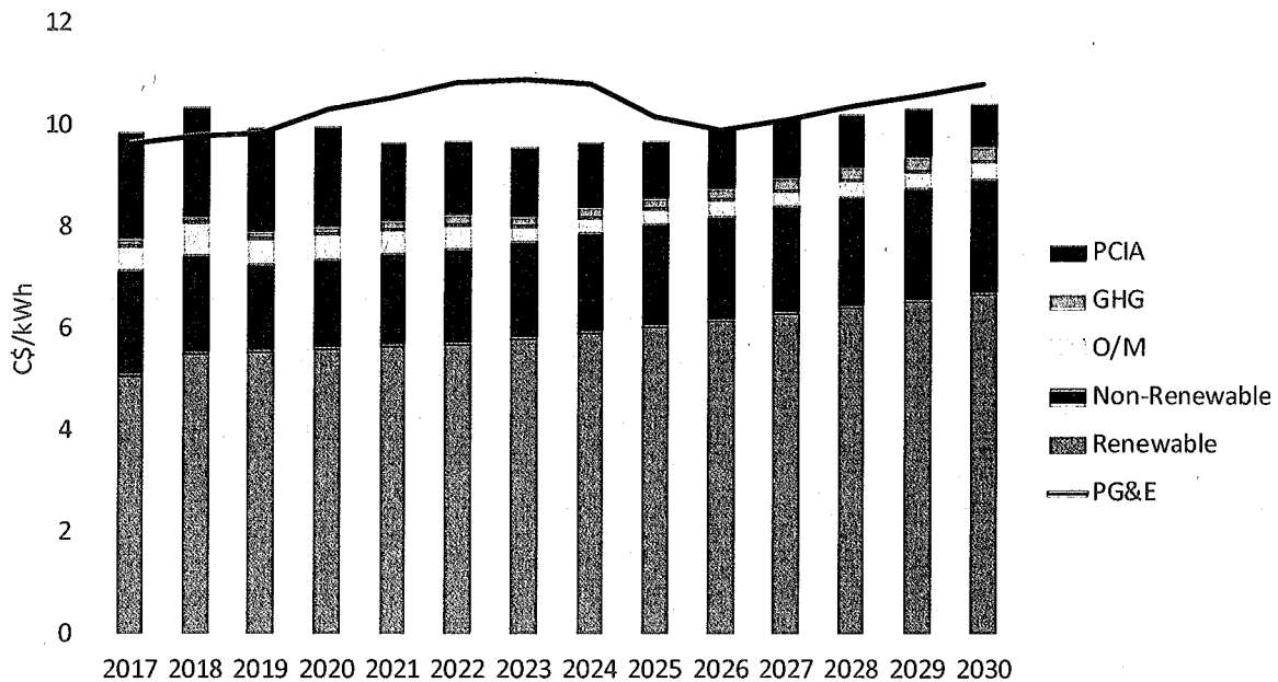
Figure 30. Scenario 2 with 50% of the Renewables Met Using In-County Generation
