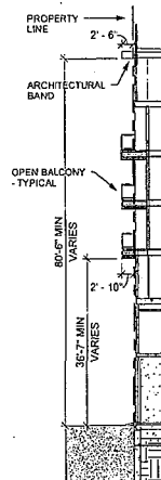
4 SECTION 4 1/16" = 1'-0"
