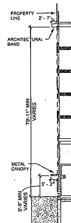
5 SECTION 5 1/16" = 1'-0"
