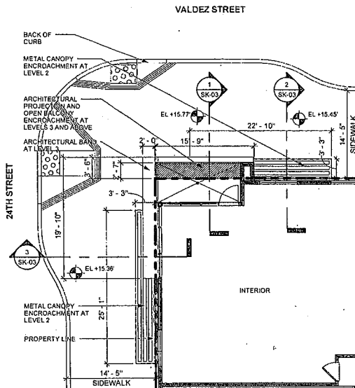
1 24TH & VALDEZ CORNER 1/8" = 1'-0"
