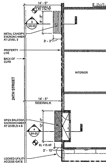
2 24TH STREET 1/8" = 1'-0"
