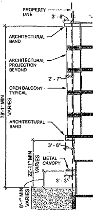
1 SECTION 1 1/16" = 1'-0"
