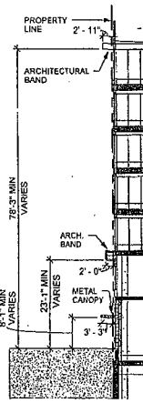
3 SECTION 3 1/16" = 1'-0"
