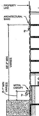
2 SECTION 2 1/16" = 1'-0"
