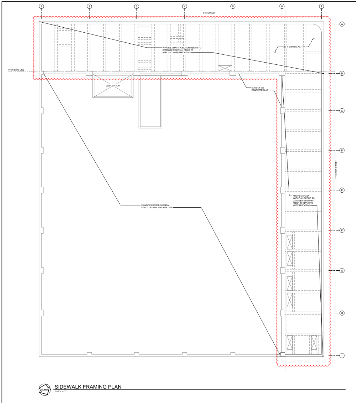
Plan View of encroaching basement below the sidewalk on 6 th Street and Franklin Street
