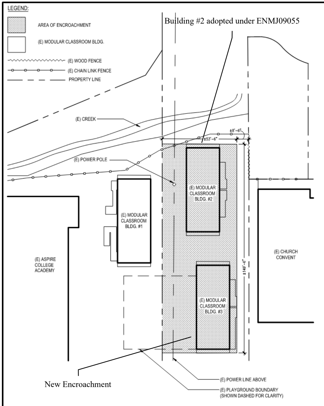
Plan View of encroaching modular classroom building #3 on unimproved portion of 81 st Avenue
