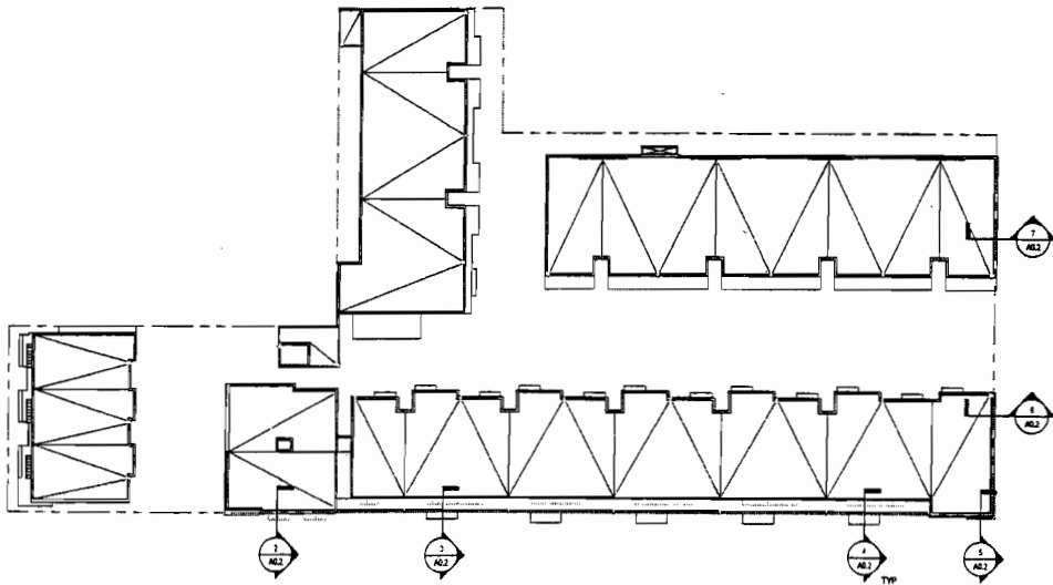
① KEY PLAN - PROJECTIONS INTO RIGHT-OF-WAY 1" = 20'-0"
