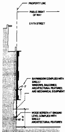
③ PROJECTION E11TH ST 1/8" = 1'-0"
