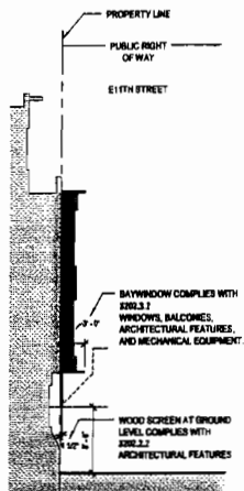
④ PROJECTION AT E11TH ST 1/8" = 1'-0"
