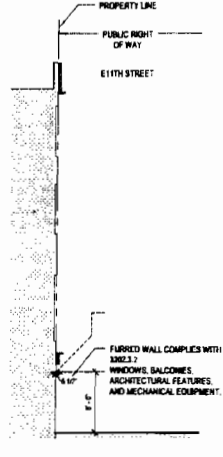
⑤ PROJECTION E11TH ST 1/8" = 1'-0"
