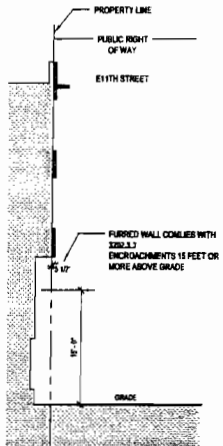
② PROJECTION E11TH ST 1/8" = 1'-0"
