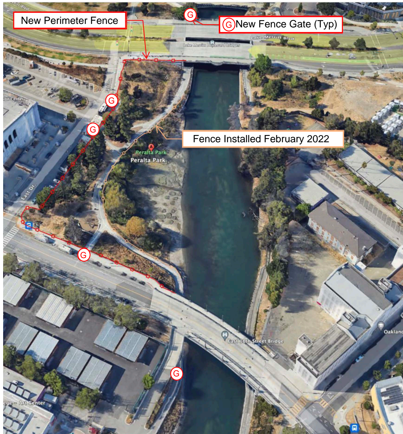
ATTACHMENT D: Peralta Park Fence Layout Diagram
