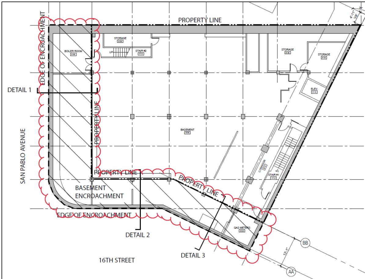
Plan View of encroaching basement below the sidewalk on San Pablo Ave and 16 th Street
