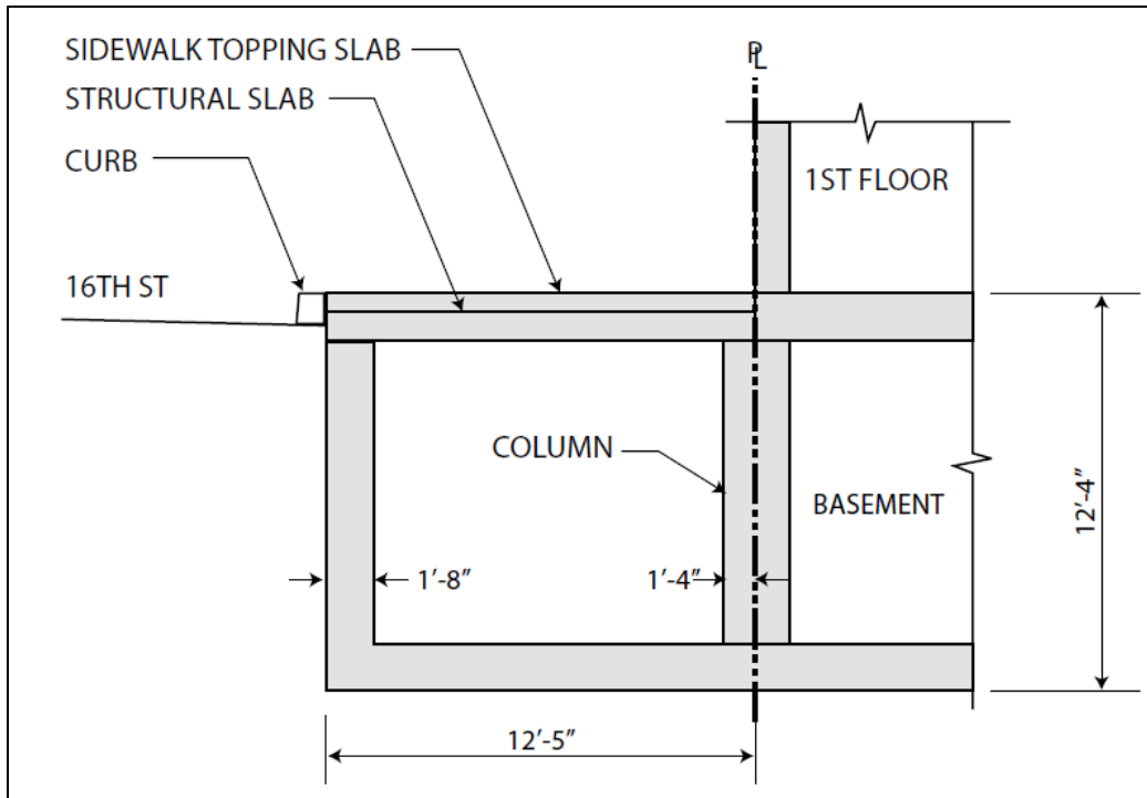
Section View of encroaching basement below the sidewalk on 16 th Street ("Detail 2" on Plan View)
