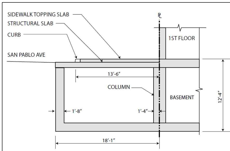
Section View of encroaching basement below the sidewalk on San Pablo Ave ("Detail 1" on Plan View)
