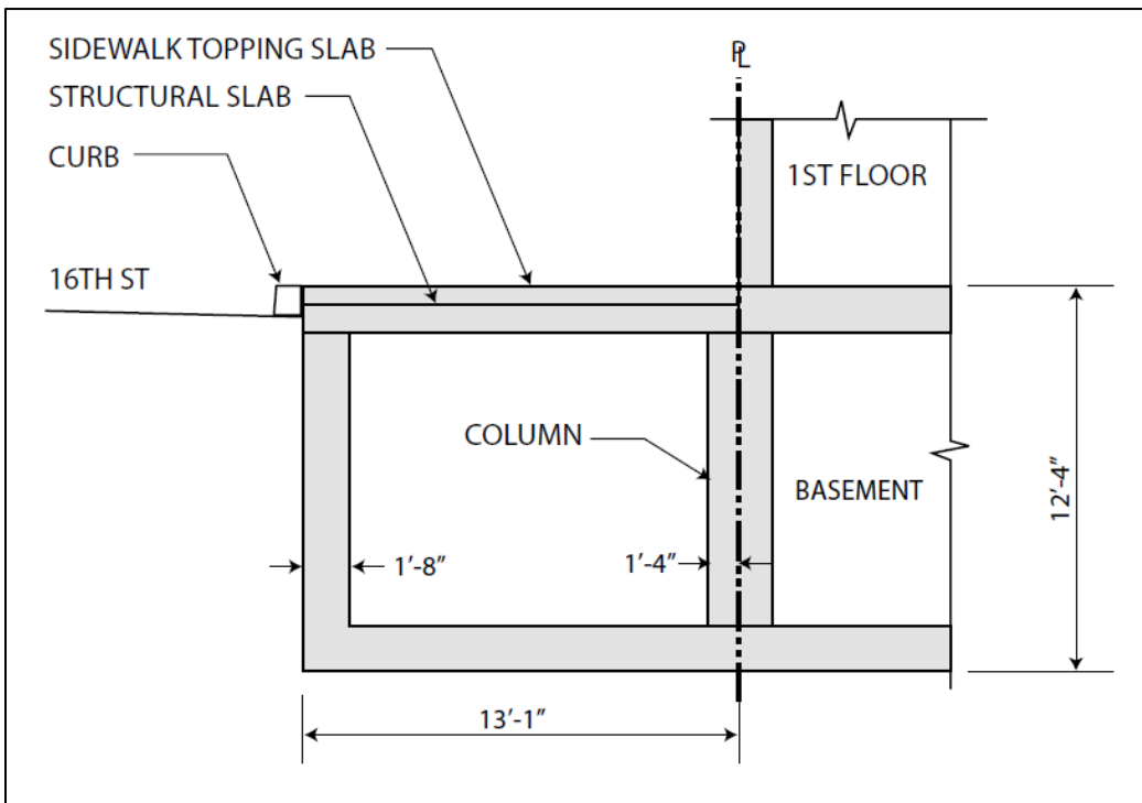
Section View of encroaching basement below the sidewalk on 16 th Street ("Detail 3" on Plan View)
