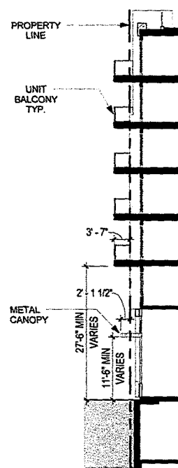
4 SECTION 4 1/16" = 1'-0"
