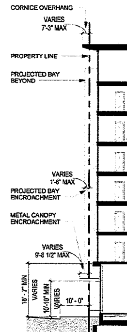
4 SECTION 4 1/16" = 1'-0"
