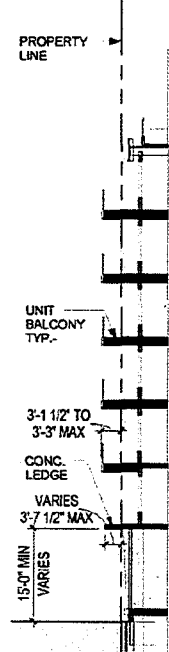
6 SECTION 6 1/16" = 1'-0"
