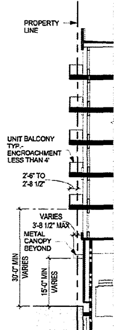
5 SECTION 5 1/16" = 1'-0"
