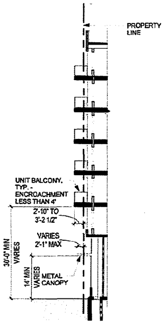
4 SECTION 4 1/16" = 1'-0"
