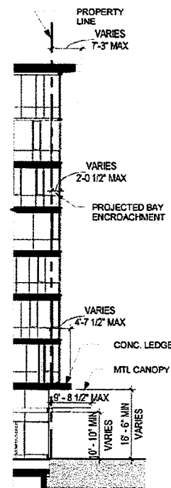
3 SECTION 3 1/16" = 1'-0"
