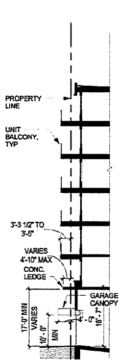
3 SECTION 3 1/16" = 1'-0"
