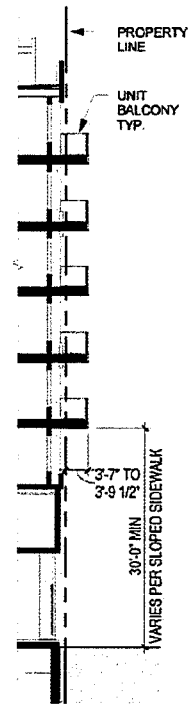
5 SECTION 5 1/16" = 1'-0"
