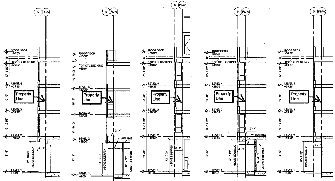
8 BAY D SECTION EPO.2 1/8" = 1'-0"
