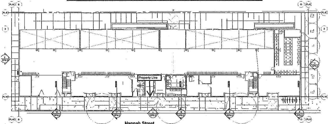
GROUND FLOOR 2850 Hannah Street
