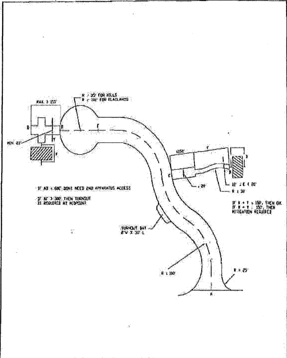
FOR ILLUSTRATION ONLY, AS A DESIGN AID ADAPTED FROM 2007 CALIFORNIA FIRE CODE- APPENDIX D 103.1
