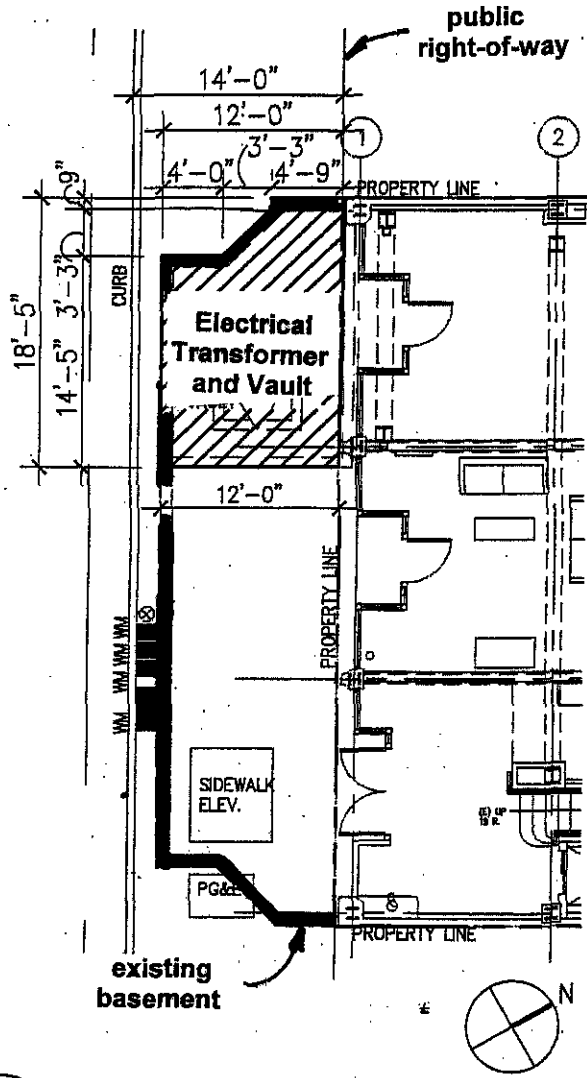
2 ENCROACHMENT PLAN 1' = 10' (ROTATED)
