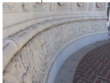
NUMEROUS MINOR SPALLS: (POSSIBLE VANDALISM) PATCH AND COAT
