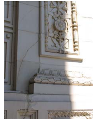
CRACK - PATCH, POSSIBLE UNIT REPLACEMENT
