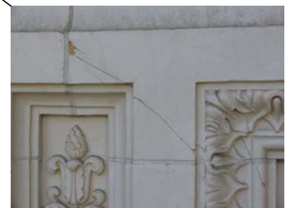
CRACK PATCH
