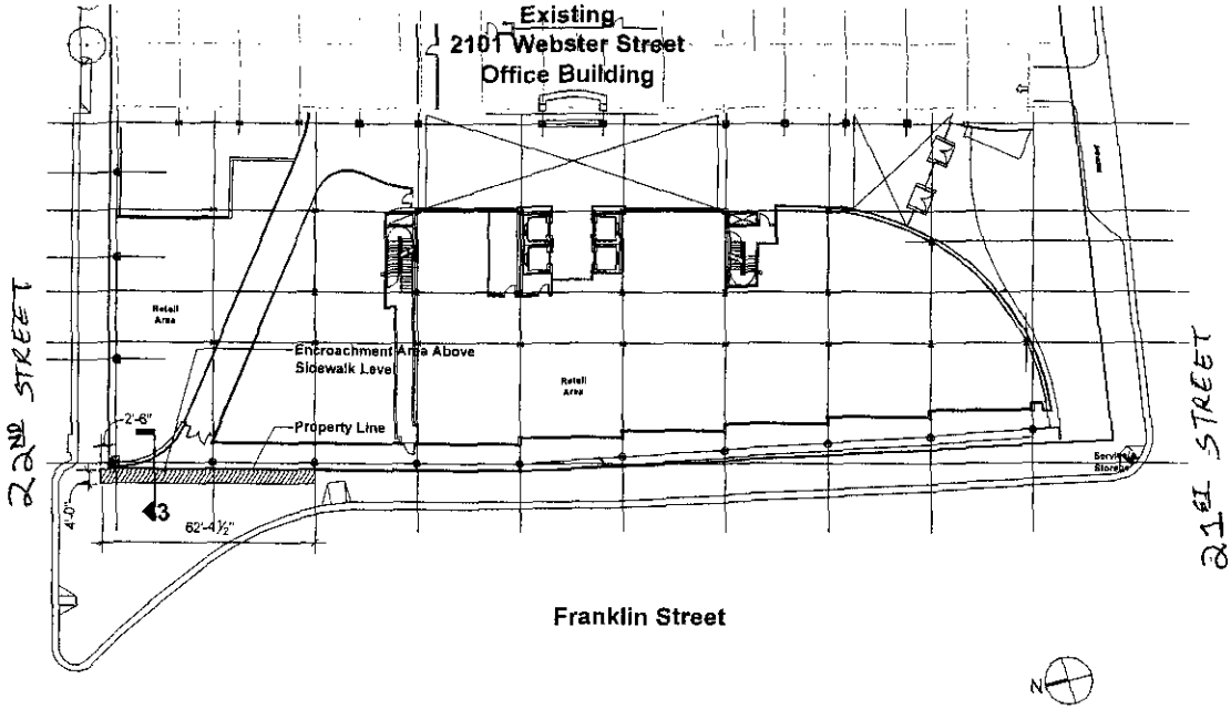
Proposed Encroachment Permit for 2100 - 2150 Franklin Street 1) First Floor & Site Plan
